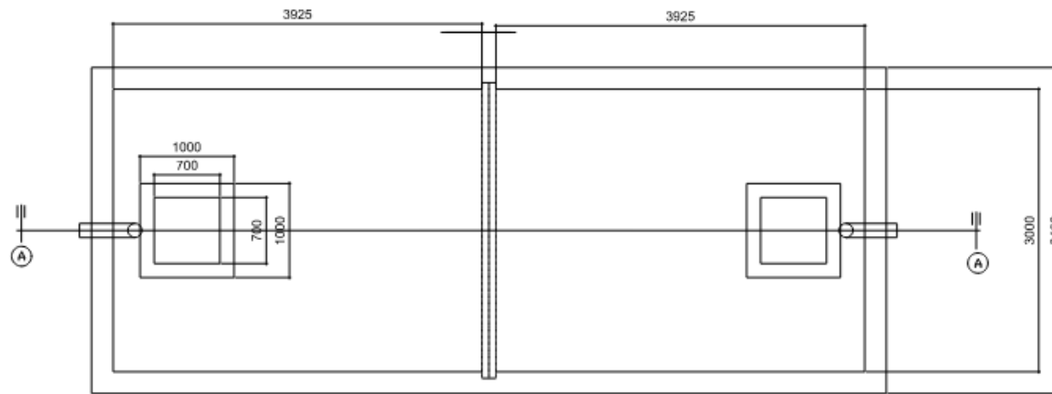
PLAN SCALE 1:30
